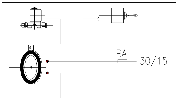
ELECTRIC DIAGRAM
